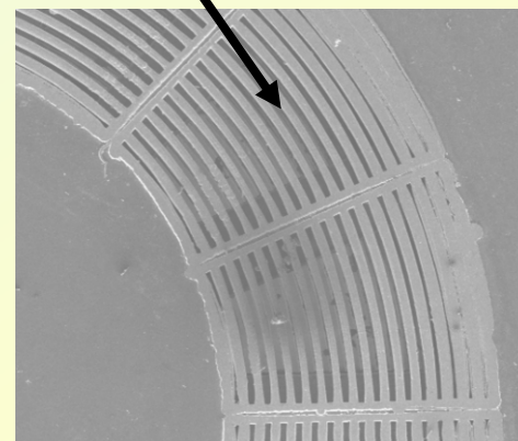
Laminated Stator
